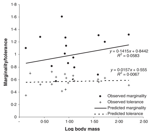
Fig. 4. Relationship between axes of specialization, marginality and tolerance, and carnivore body mass (log transformed).
